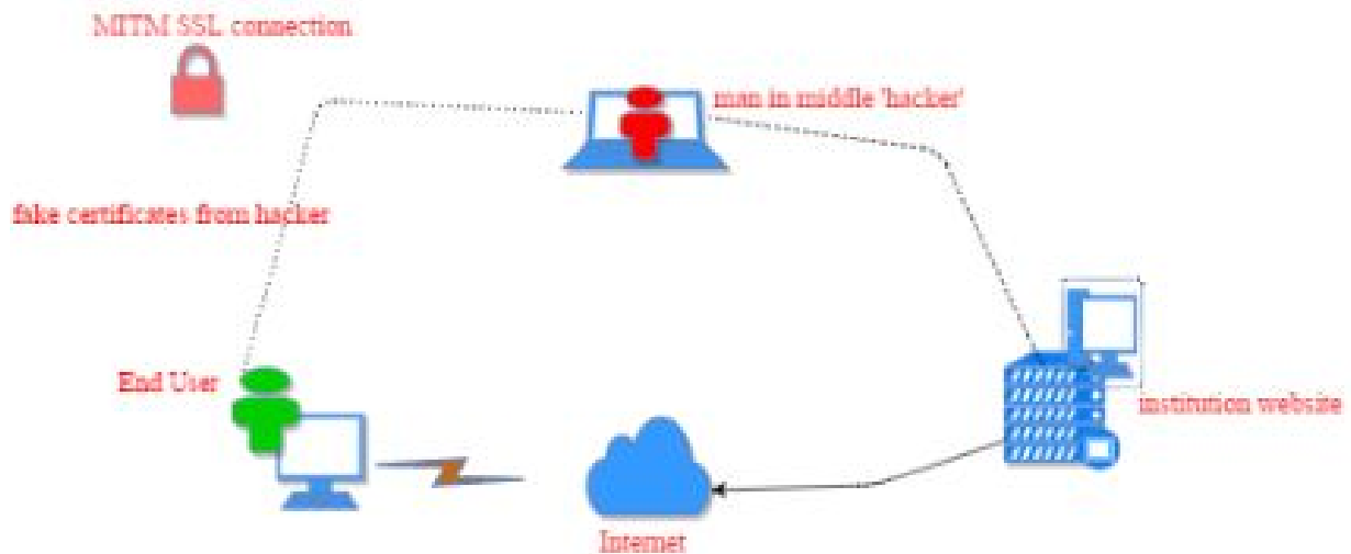
Fig 4. Man-In –Middle-Attack
