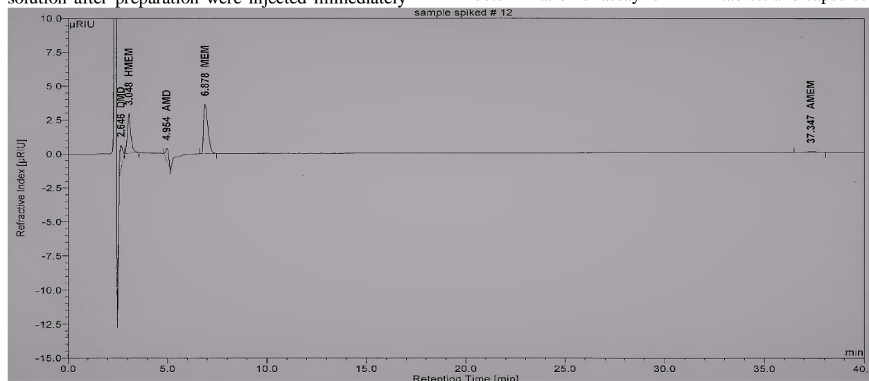
Fig. 2: Chromatogram of Memantine HCl along with diluents, placebo and known impurities.
